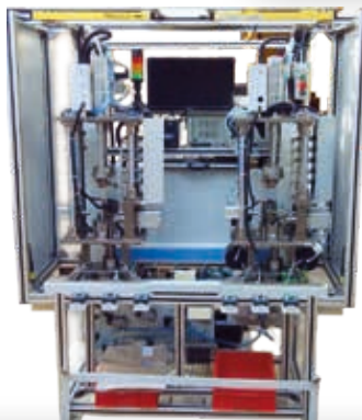
Hydraulic ABS Testing Station 📍 Jamshedpur, Jharkhand
